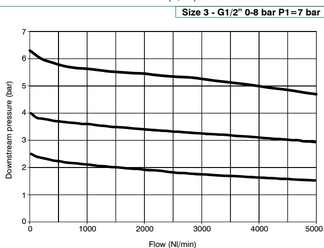
Adjustment characteristic
