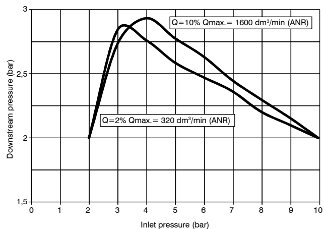
Adjustment characteristic
