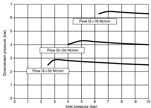
Adjustment characteristic
