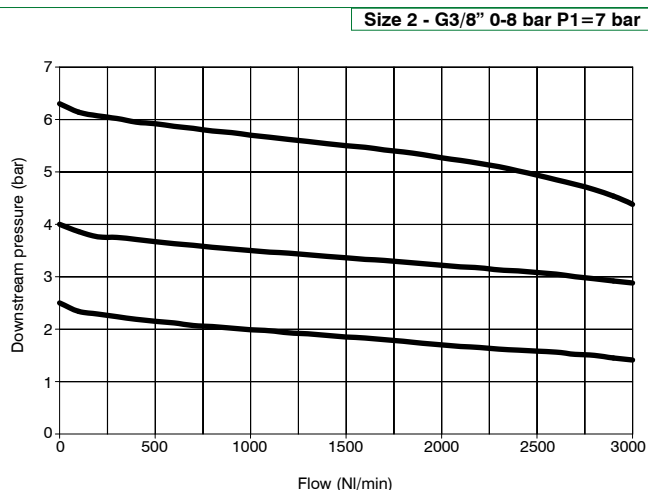
Adjustment characteristic
