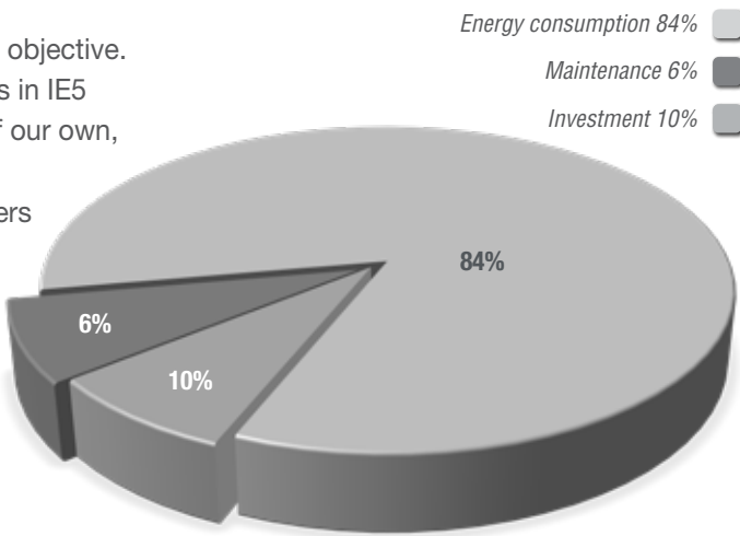
The graph represents the total life cycle costs breakdown of a 37 kW fixed speed compressor, over 5 years of use, considering 4000 working hours per year and an energy cost of about 0.17 €/kWh.
