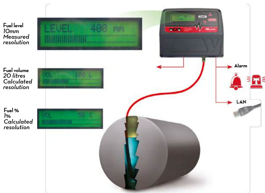
SSM 2.0 SOFTWARE
