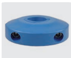
Hose stop with six exchangeable inserts. Hose \varnothing 10 - 34 mm
