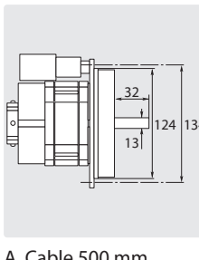
Flange with pump shaft 32 mm
