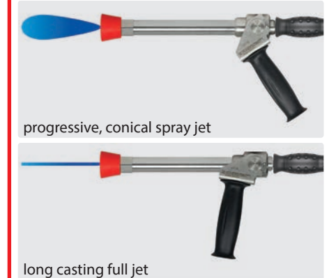
1/2" F. Stainless steel. Longcast lance 350 mm with insulation ST-29 Cool & Compact 330 mm, gun easyfarm365+, grip aside and nozzle protector made out of plastic without nozzle. Max. 250 bar / 60 l/min / 100 °C
