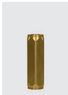
1/4" F. Brass. I 62 mm. Opening pressure 0.05 - 0.1 bar. Max. 150 bar / 90 °C
