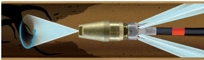
Hardened stainless steel. 6 M5 threads for nozzle inserts (see table below)
