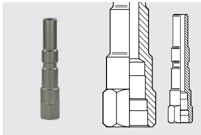
KW : 1/4" F. Stainless steel. SW 17. For lances with vented handle
