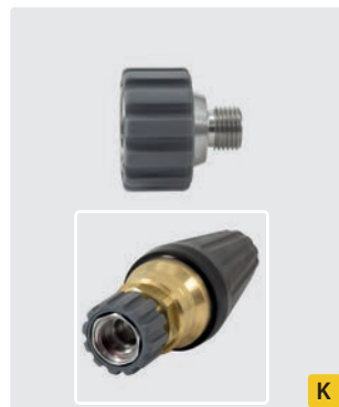
TR20 F : 1/4" M. Stainless steel. Max. 400 bar / 150° C
