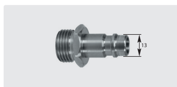
Plug : M. Stainless steel. Max. 150 bar / 90 °C
