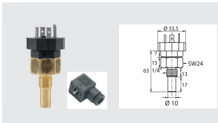
Bimetal temperature switch with plug. Switching point accuracy \pm 5 °C. Reset temperature 15...40K. Switching voltage up to AC 250 V / 2A. Max. 10 bar in the inlet. Switch 1/4" M
