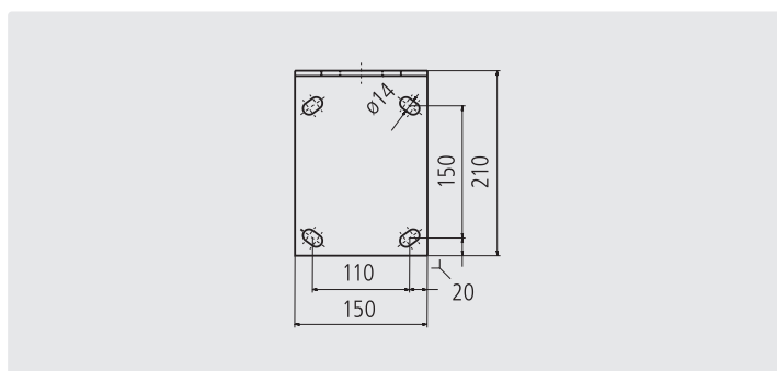
Wall plate
