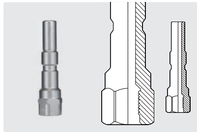
KW : 1/4" F. Stainless steel. SW 19. Plug for moulded handles
