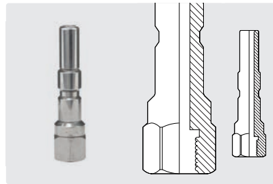
KW : 1/4" F. Polished stainless steel. SW 19. For moulded handles. Plug for aluminium washer
