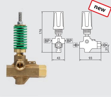
ST-265 with green spring (240 bar)
