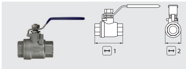
Stainless steel V2A / AISI 304. Ball stainless steel. Max. 140 bar / 60 °C
