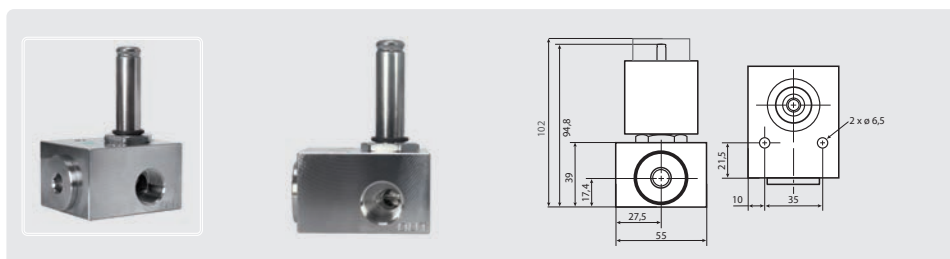
Stainless steel. Viton. Pressure range 0 - 160 bar. Without coil. Max. 90 °C
