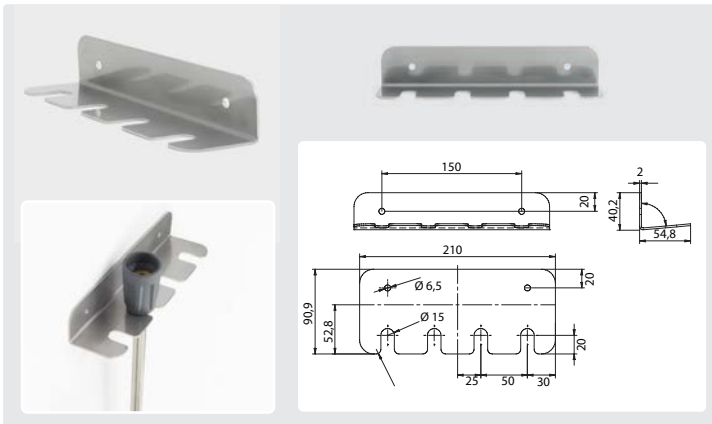
Stainless steel. Wall mount for 4 lances with coupling KW
