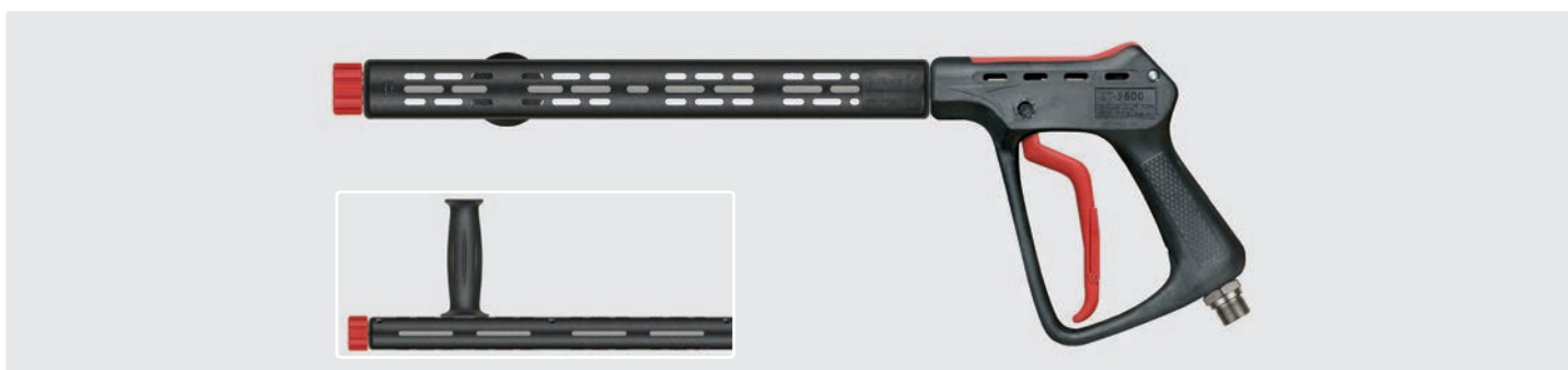
Professional ultra high pressure gun with extension ST-9 380 mm, grip and M22 F. Max. 500 bar / 80 l/min / 150 °C
