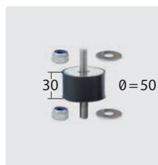
Rubber buffer type A. M10 x 28. Incl. Screws and washers. Steel or stainless steel and elastic natural rubber 55°. Spring stiffness: 500 N / mm. Load: 2,000 N
