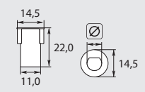
Coupling for shaft \varnothing 8 mm long
