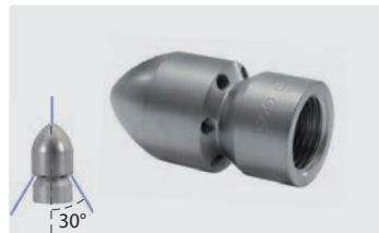
1/2" F. Outside \varnothing 30 mm. rear jets, with front jet
